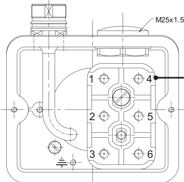
SIGNAL CONNECTOR
